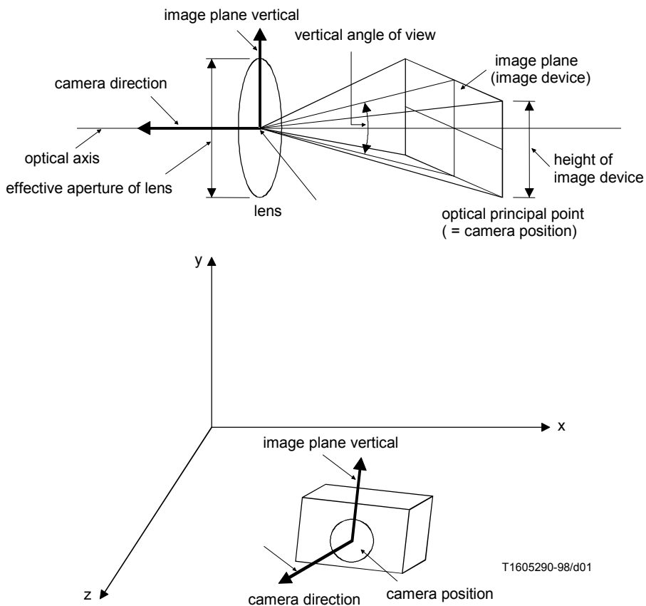
Figure 6-23 — Camera parameters
