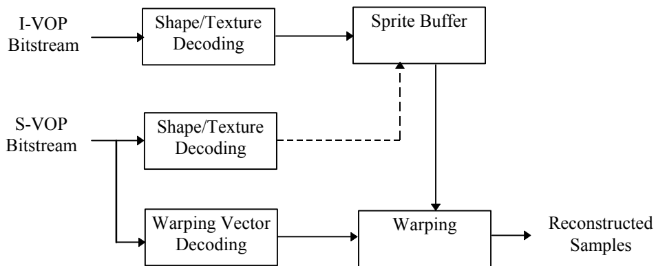
Figure 7-121 — The sprite decoding process
