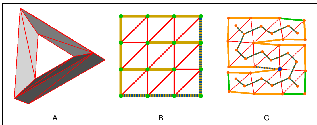
Figure O.1 — Example of Topological Surgery on a torus.
