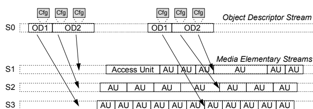
Figure K.3 — Integrated Systems and Visual approach
