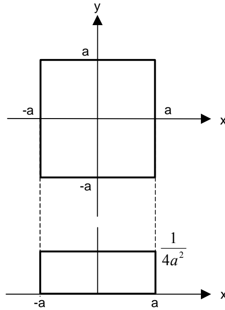
Figure 6-24 — Defocusing filter
