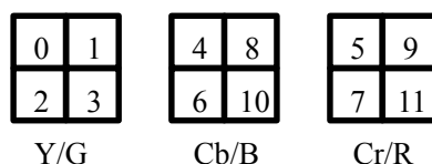
Figure 6-10 — 4:4:4 Macroblock structure
