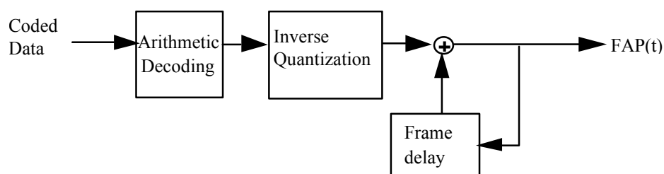
Figure 7-80 — FAP decoding
